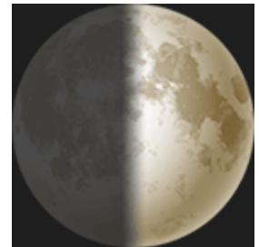
First Quarter November 27 11:22 UTC
