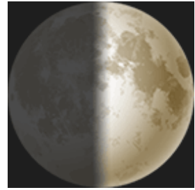
First Quarter November 27 11:22 UTC
