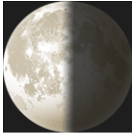
Last Quarter November 12 02:03 UTC
